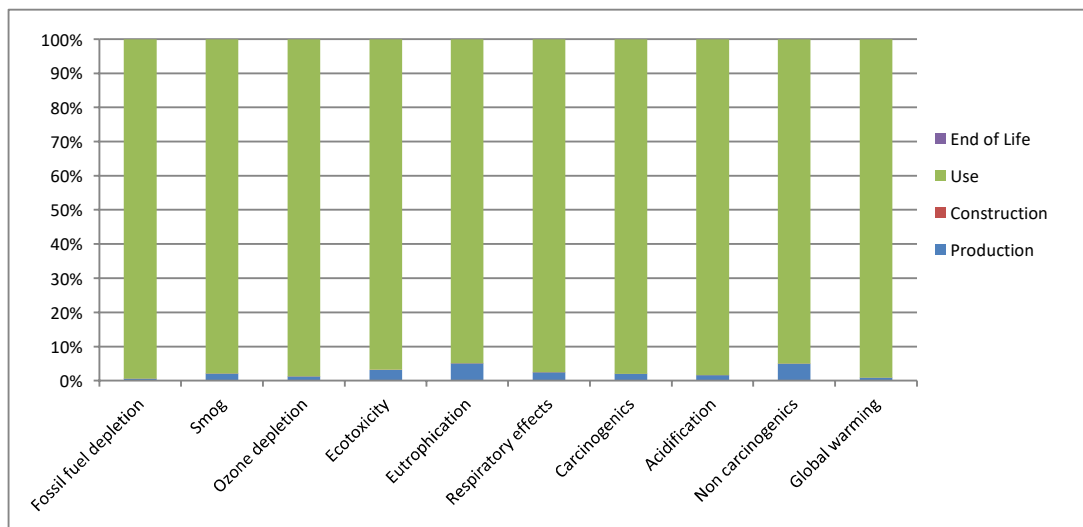
Figure 13. LCIA results for the average of T28S32E and T27S32E– relative results
