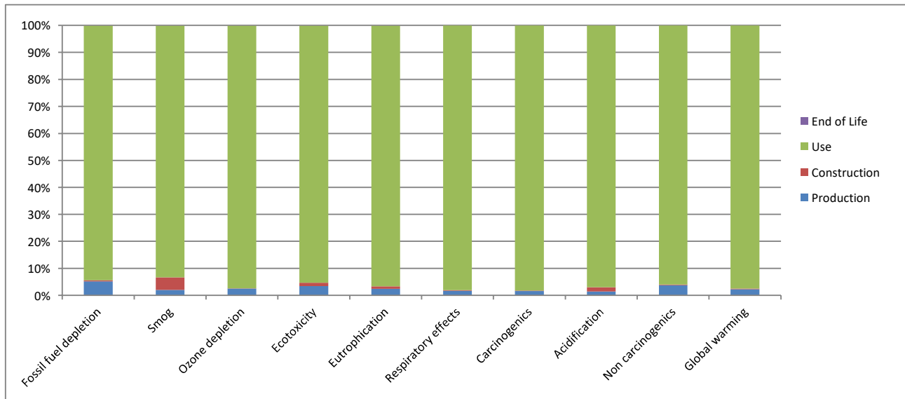
Figure 6. LCIA results for Drake 1G– relative results
