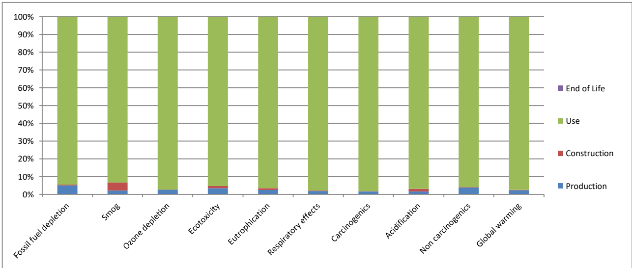
Figure 5. LCIA results for Drake HET– relative results
