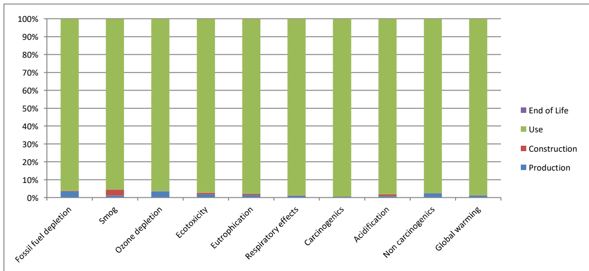
Figure 10. LCIA results for Ultramax HET (MS604124CEFG) -- relative results
