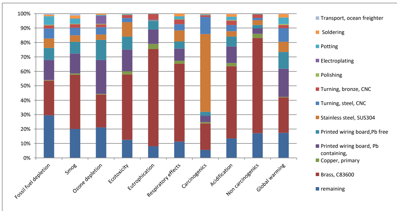
Figure 28. Cradle-to-gate impacts for TET2UB(X) – relative results
