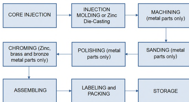
Figure 3. Faucet and flush valve manufacturing process flow
