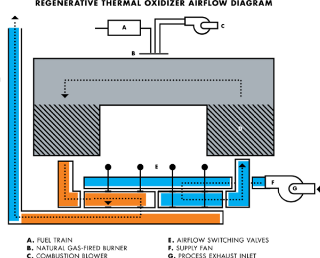
REGENERATIVE THERMAL OXIDIZER AIRFLOW DIAGRAM
