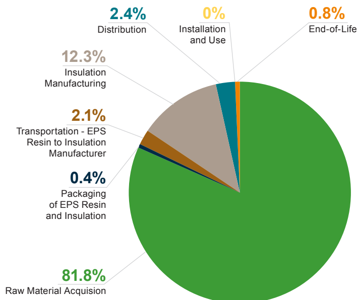
Figure 3: Cumulative Energy Demand for EPS Insulation
