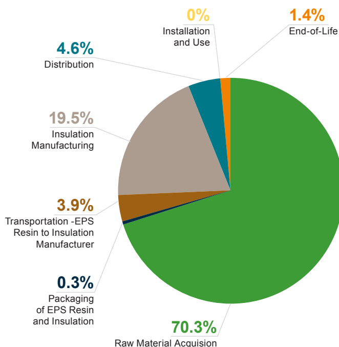
Figure 4: Global Warming Potential Results for EPS Insulation
